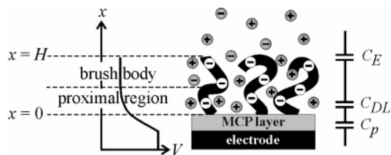
Figure 4. Model used in the derivation of the charging response of a polyelectrolyte brush. The expected potential profile is schematically indicated on the left, and the equivalent circuit description is shown on the right.
